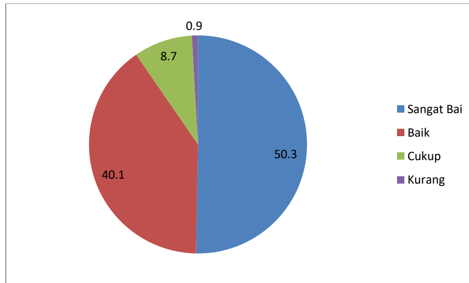
Gambar 5: Responsiveness
